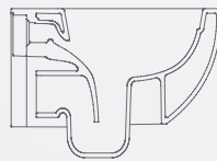
CLEAN FLUSH HUNG WC Art. 5520/CL - Pag. 69
